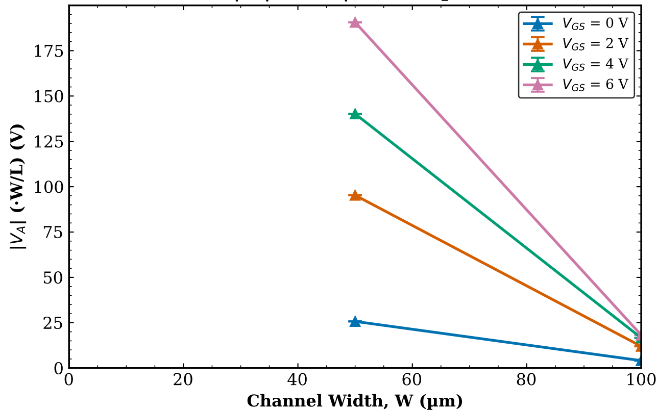
TFT3 Transistor 1 |V_A| vs W | L = 40\text{ }\mu\text{m}
